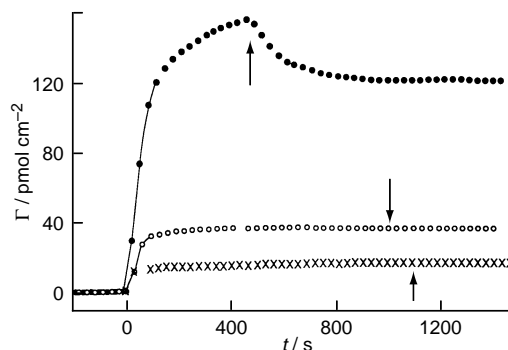
Fig. 1 Representative experimental data: (×) 1 , c_b = 4 \mu M; (○) 2 , c_b = 2 \mu M; (●) 2 , c_b = 200 \mu M. Bulk flow was switched to the ruthenadendrimer solution at t = 0 . The arrows denote when the flow reverted to pure buffer.
